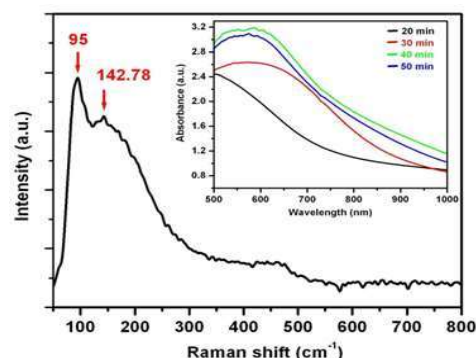
Fig. 2. Typical Raman spectra of PbS thin films. (Inset figure shows plot of absorbance versus wavelength)
